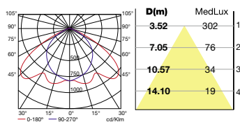
TL5 G5 1x54W double parabolic
