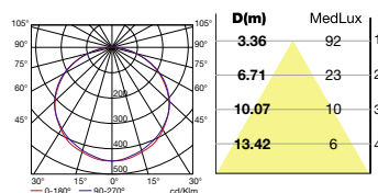
TL5 G5 1x54W polycarbonate
