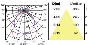
TL5 G5 2x54W double parabolic
